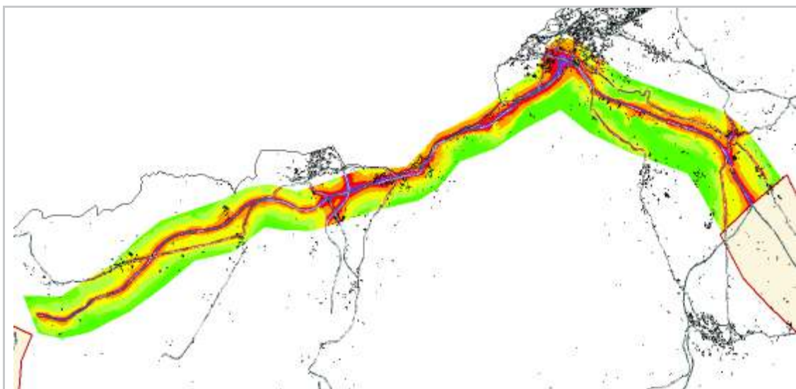
Illustration 57: Second sub-section – Vuache Tunnel – Sciontrier. Horizontal mapping of noise levels (LDEN (dB(A))) calculated at 4 meters above ground.
