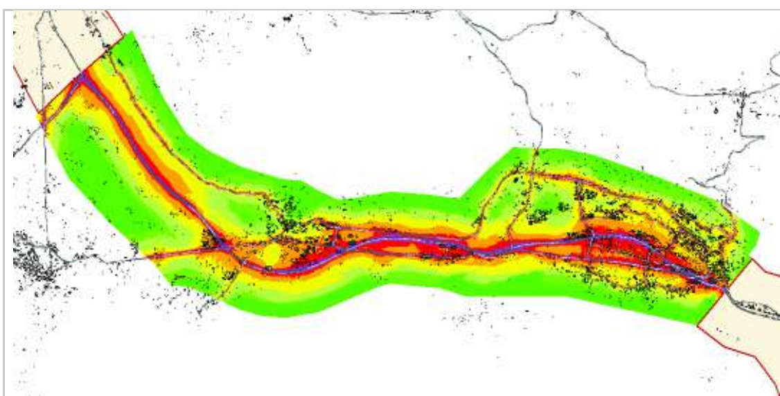
Illustration 58: A40 Sciontrier – Cluses. Horizontal mapping of noise levels (LDEN (dB(A))) calculated at 4 meters above ground.
