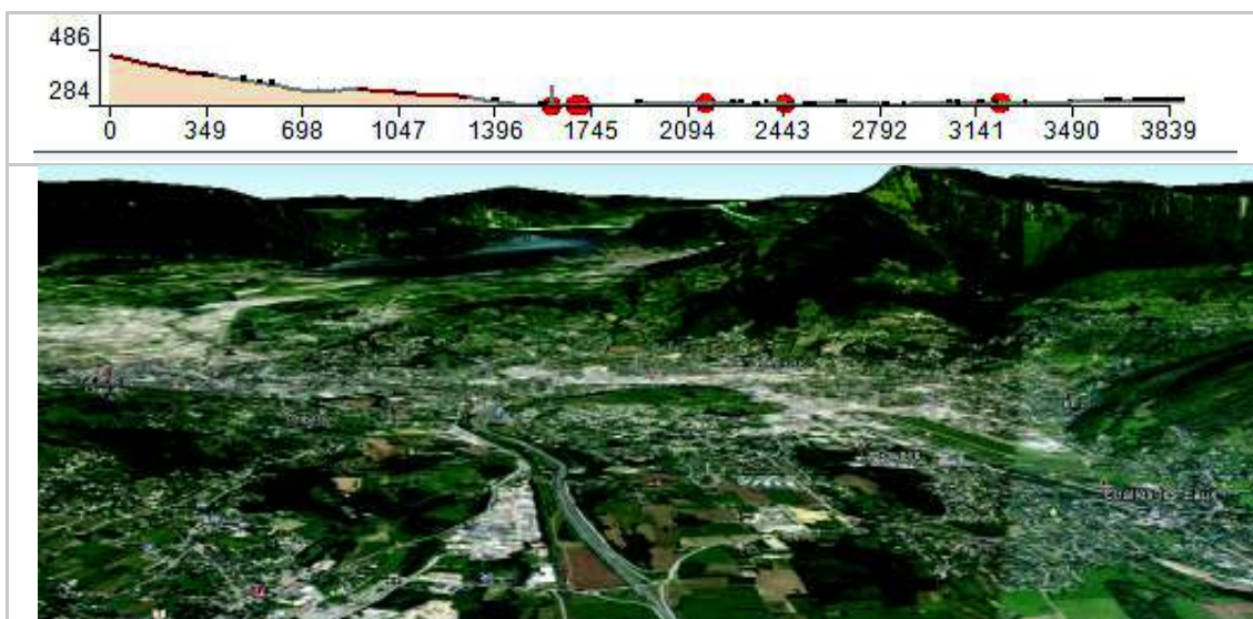
Illustration 31: A43 A41-A43 - Aiton. Typical cross-profile of this section. Red dots mark the location of road infrastructure modelled as acoustic sources. Horizontal and vertical scales (in meters) and aerial view (GoogleEarth) of the area.
